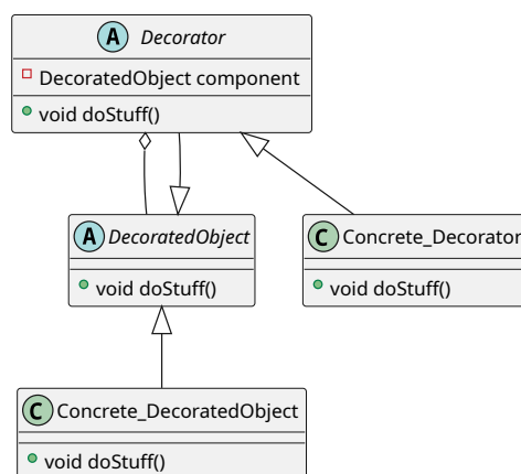
Figure 313: Diagram of the Decorator Pattern
